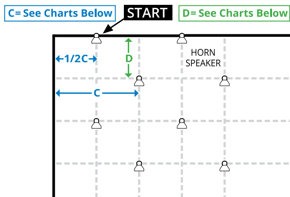
Horn Speaker Layout
