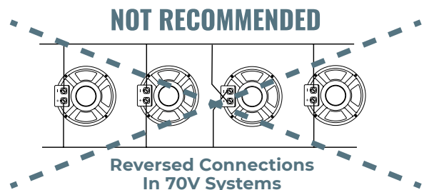
Reversed polarity in one speaker causes the sound between the speakers to be cancelled, mostly affecting the bass
